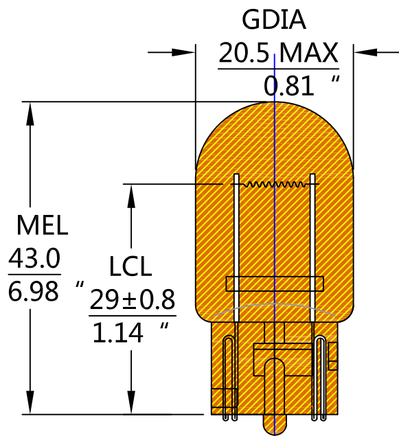
0° VIEW
