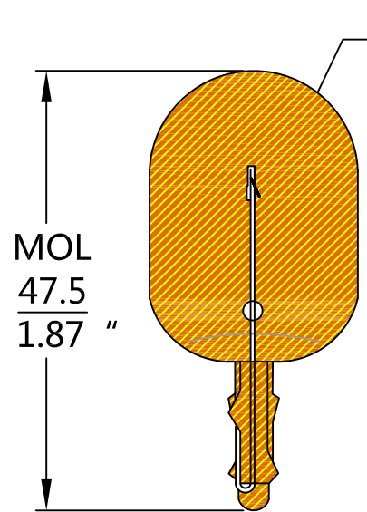
90° VIEW
